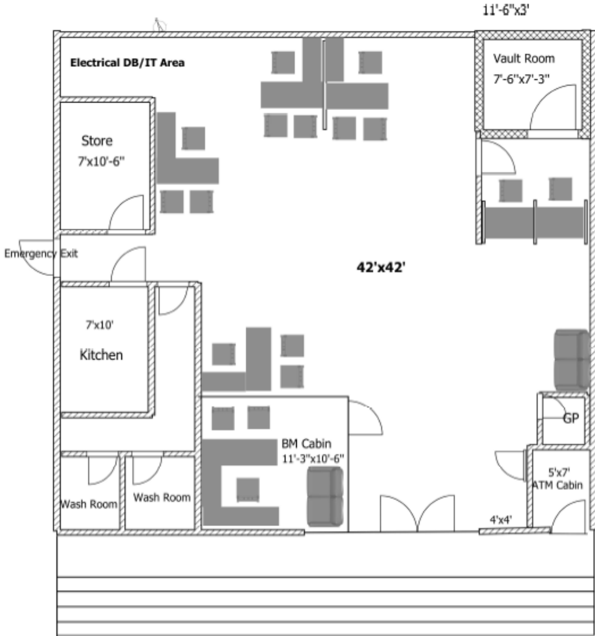
PROPOSED SATGRAH BRANCH Relocation
